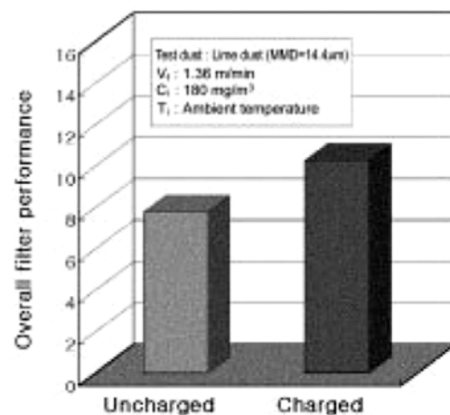
Fig. 6. Filter performance.
