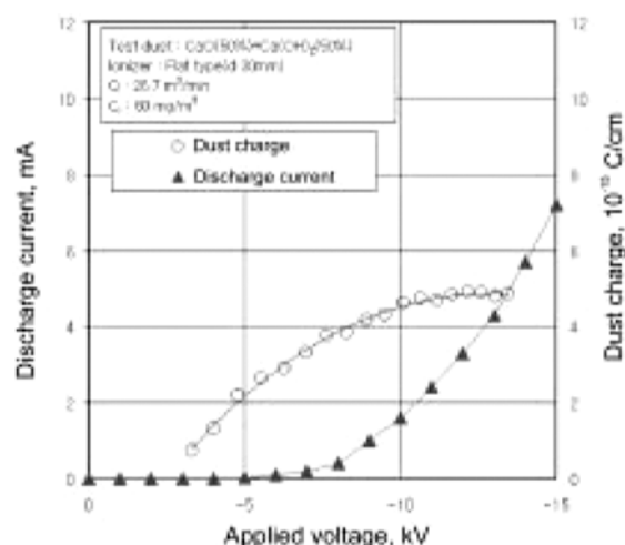
Fig. 3. Discharge and dust charge characteristics of dust precharger.
